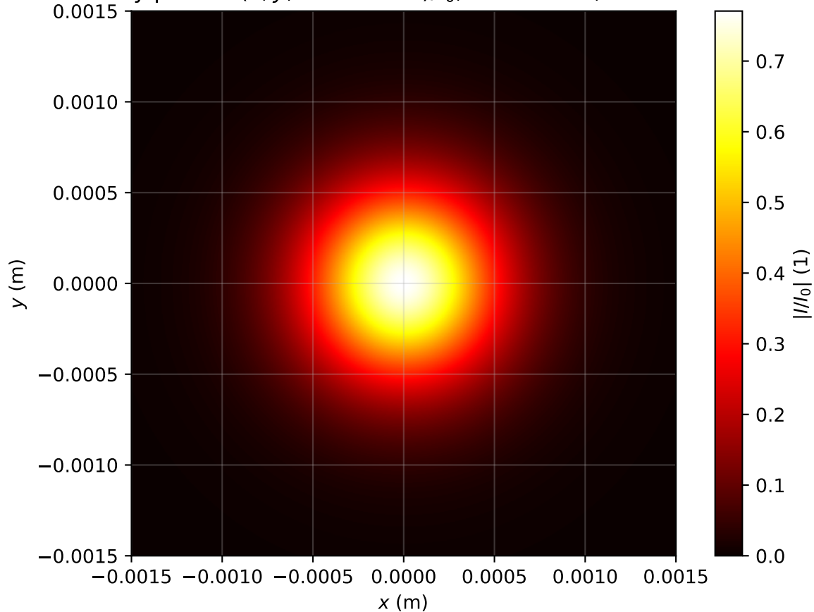
Intensity profile I(x, y, z = 2.627m)/I_0 , Pin=0.6Pcr, artificial time
